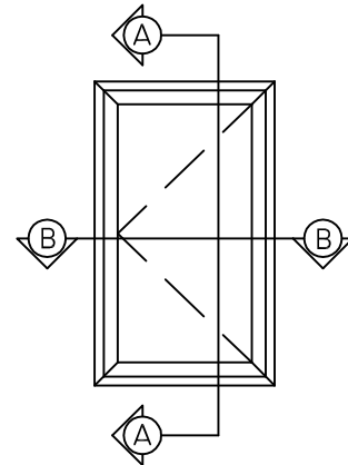
VinylPro 2000™ CASEMENT WELDED ASSEMBLY
