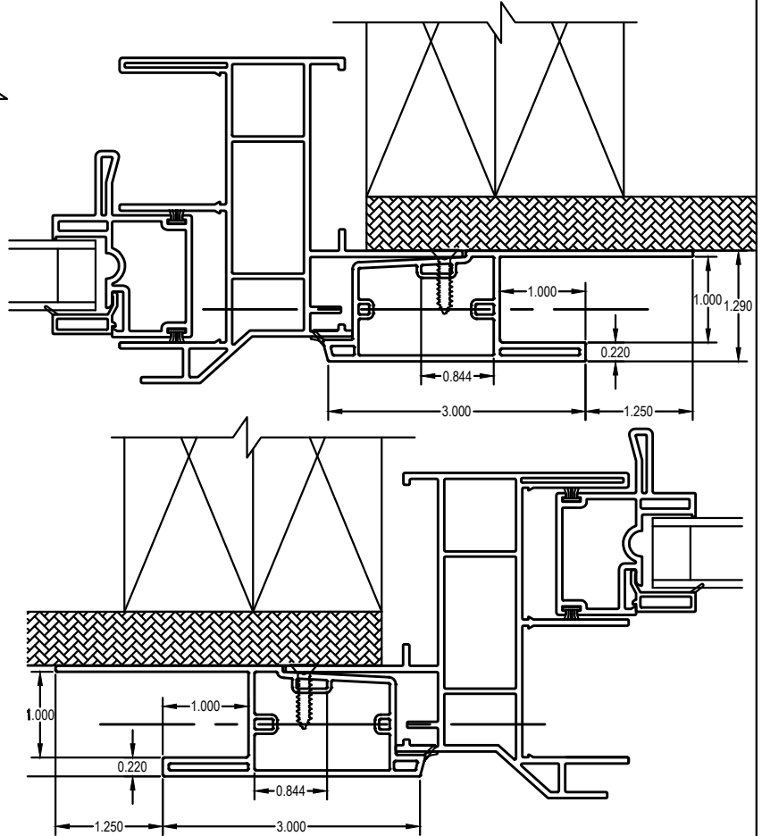
SLIDER JAMB WITH NEW ENGLAND FLAT CASING
