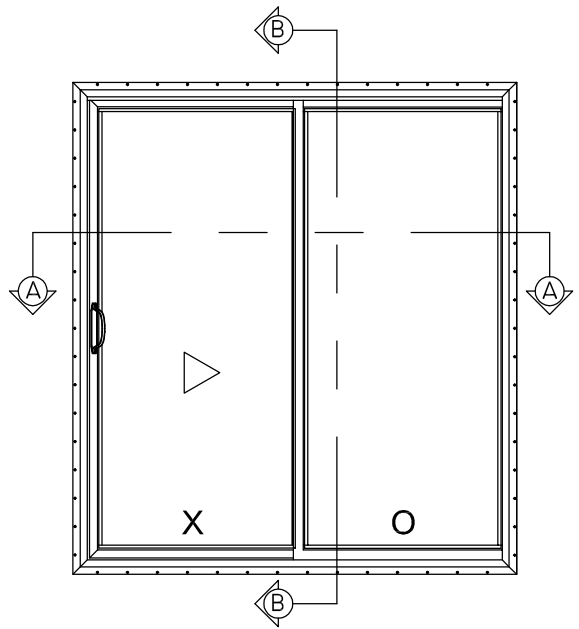
NUCON ® SLIDING PATIO DOOR WELDED ASSEMBLY
